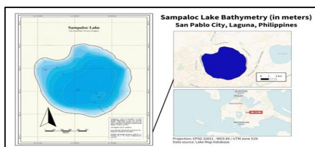
Figure 3 Sampaloc Lake Bathymetry (in meters)
