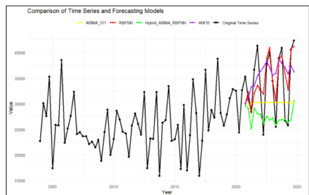
Figure 1 Graphical presentation of model's performance in predicting test set. Green (Hybrid), Red (RBFNN), Violet (ANFIS), Yellow (ARIMA)
