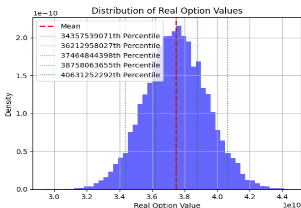
Figure 9 The distribution Plot of the Real Option Value; as computed through the Monte Carlo Simulation.
