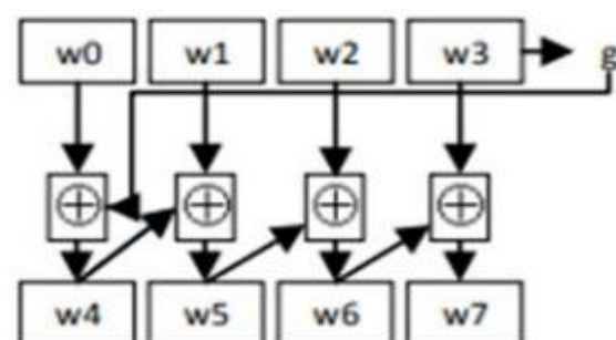
Figure 2 Key expansion algorithm
