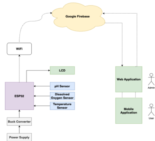
Figure 3 Functional Block Diagram of Utilizing Data-Driven Approaches for Water Quality Monitoring in Inland Fisheries
