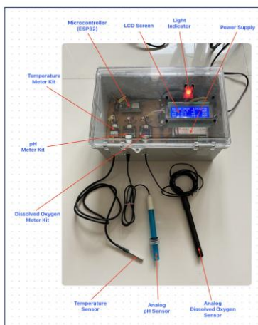
FIGURE 8 The water quality monitoring prototype
