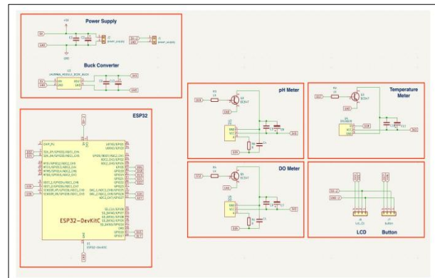
FIGURE 9 Schematic Diagram of the Water Quality Monitoring Device
